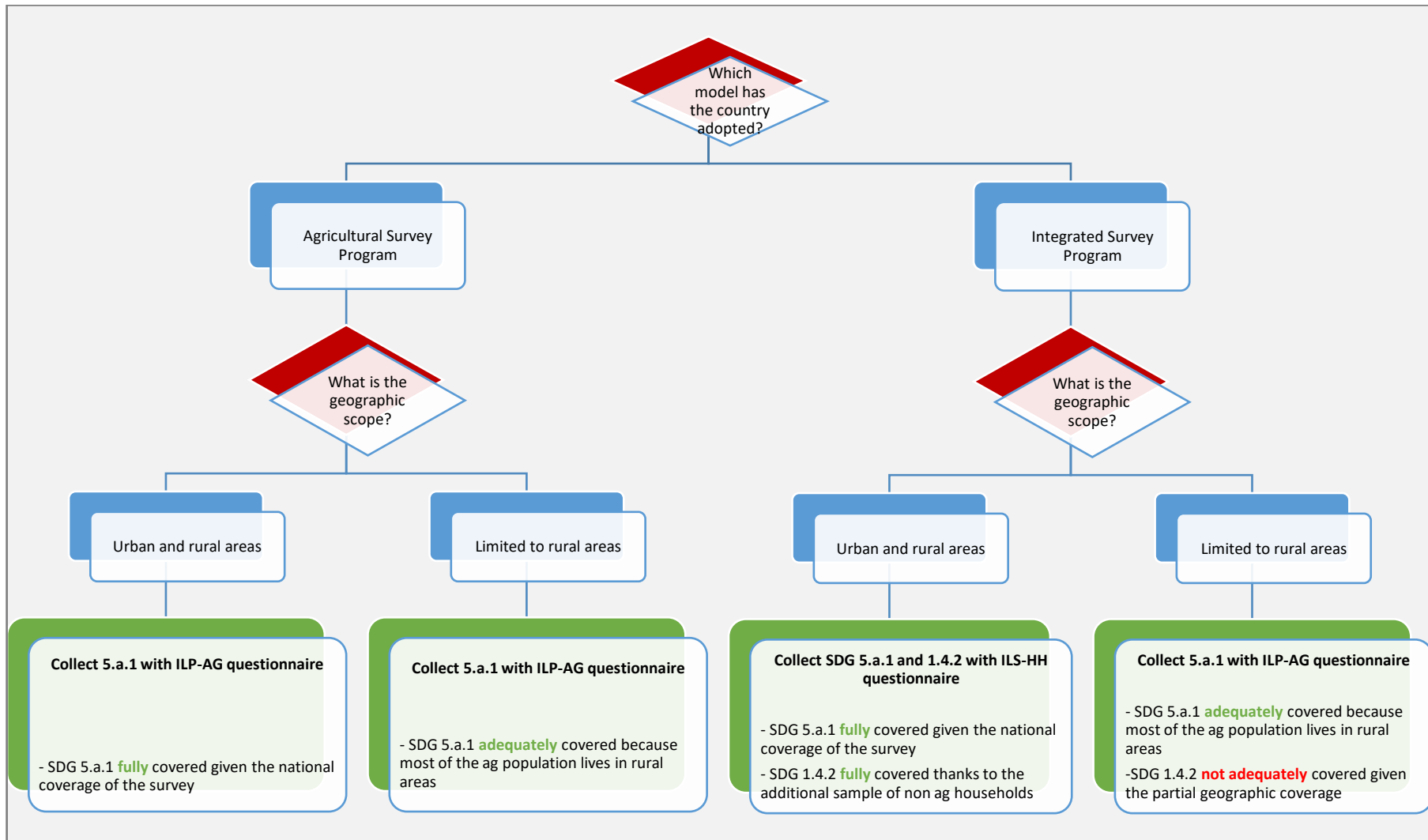
FIGURE 5 – DECISION TREE
